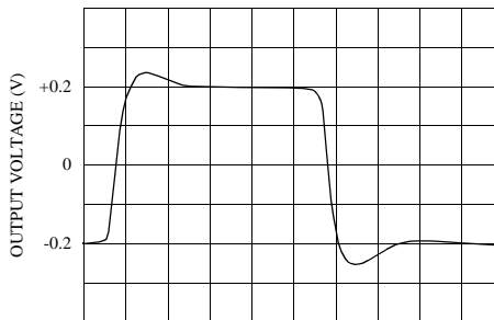
Small Signal Pulse Response (Split Supply)
