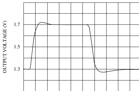
Small Signal Pulse Response (Single Supply)
